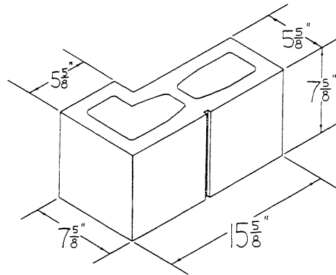
6×8×16 "L" RETURN BLOCK— ONE SCORE
