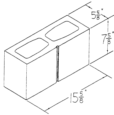
6×8×16 DOUBLE SOLID END—ONE SCORE
