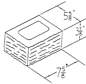
6×4×8 SPLIT BLOCK HALF— ONE FACE, ONE END
