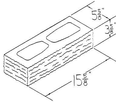
6×4×16 SPLIT BLOCK— ONE FACE, ONE END
