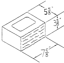
6×4×8 SPLIT BLOCK HALF—ONE FACE
