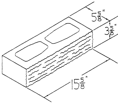
6×4×16 SPLIT BLOCK—ONE FACE
