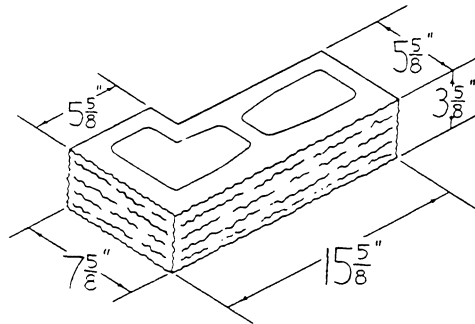
6×4×16 "L" RETURN SPLIT BLOCK— ONE FACE, ONE END
