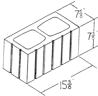
8×8×16 FIVE SCORE—ONE FACE, ONE END (AVAILABLE IN TWO FACE, TWO END)
