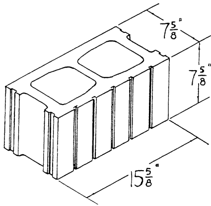
8×8×16 FIVE SCORE—ONE FACE (AVAILABLE IN TWO FACE)
