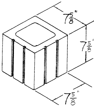
8×8×8 FIVE SCORE HALF BLOCK— ONE FACE, ONE END (AVAILABLE IN TWO FACE, ONE END)
