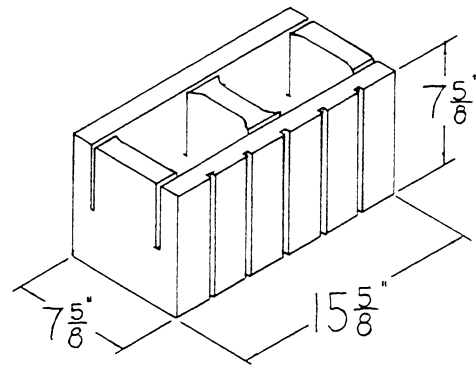
8×8×16 FIVE SCORE KNOCK OUT LINTEL/BOND BEAM (AVAILABLE IN TWO FACE)
