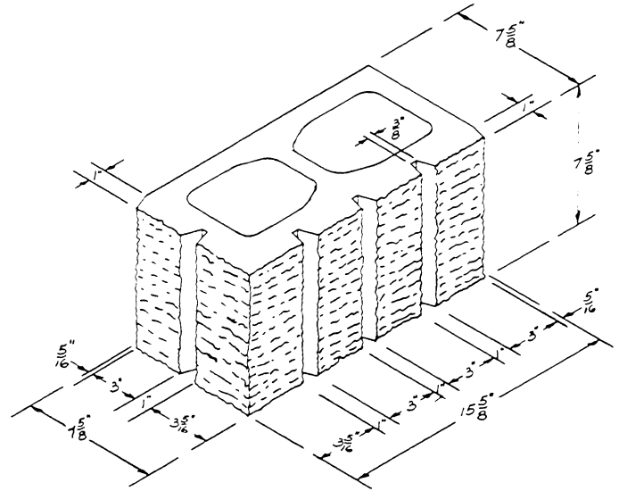
8 × 8 × 16 VEE THREE FLUTE SPLIT ONE FACE ONE END (AVAILABLE IN TWO FACE. ONE END)
