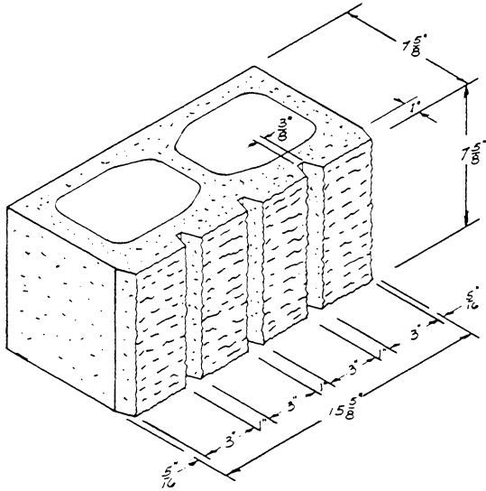
8 × 8 × 16 VEE THREE FLUTE SPLIT ONE FACE (AVAILABLE IN TWO FACE)
