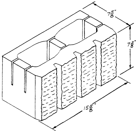
8 × 8 × 16 VEE THREE FLUTE SPLIT ONE FACE KNOCK OUT LINTEL/BOND BEAM (AVAILABLE IN TWO FACE)
