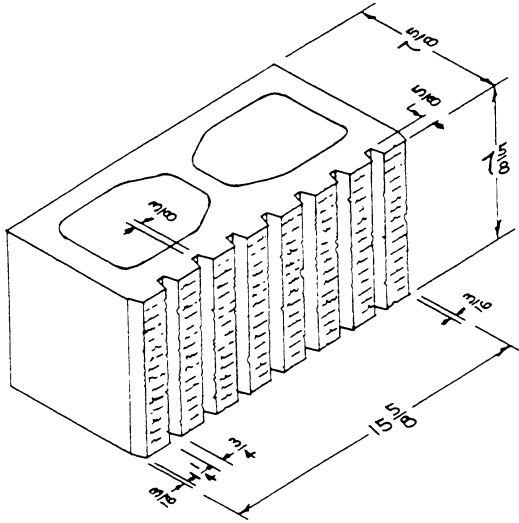
8 × 8 × 16 VEE SEVEN FLUTE SPLIT ONE FACE (AVAILABLE IN TWO FACE)
