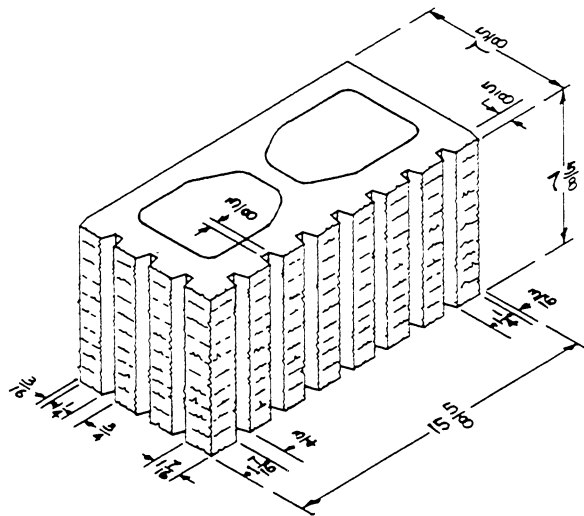
8 × 8 × 16 VEE SEVEN FLUTE SPLIT ONE FACE ONE END (AVAILABLE IN TWO FACE, TWO END)
