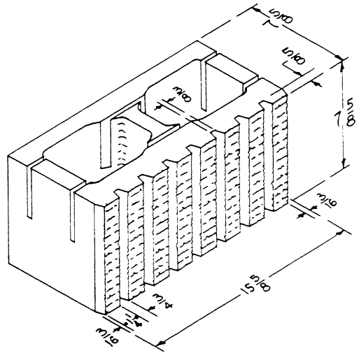
8 × 8 × 16 VEE SEVEN FLUTE SPLIT ONE FACE KNOCK OUT LINTEL/BOND BEAM (AVAILABLE IN TWO FACE)
