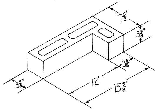
4 × 4 × 16 "L" RETURN BLOCK
