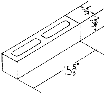
4 × 4 × 16 DOUBLE SOLID END
