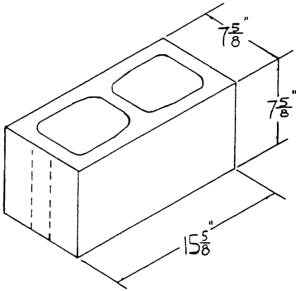
8×8×16 DOUBLE SOLID END (ALSO AVAILABLE IN SASH BLOCK)
