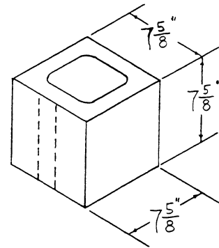
8×8×8 HALF BLOCK (ALSO AVAILABLE IN SASH BLOCK)
