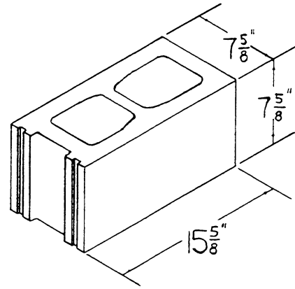
8×8×16 SINGLE SOLID END
