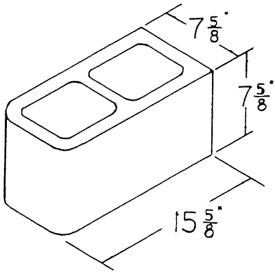
8x8x16 BULL NOSE BLOCK ONE END
