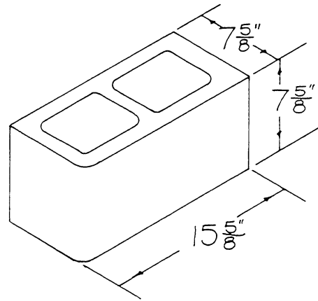
8x8x16 BULL NOSE BLOCK ONE CORNER
