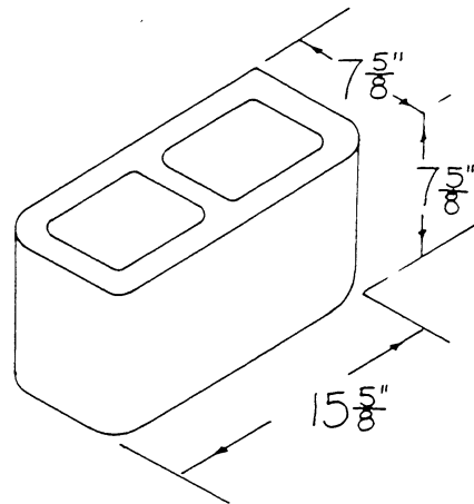
8x8x16 BULL NOSE BLOCK FACE AND END
