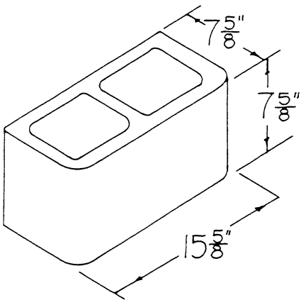
8x8x16 BULL NOSE BLOCK ONE FACE
