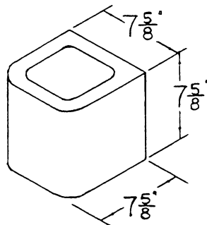
8x8x8 BULL NOSE HALF BLOCK
