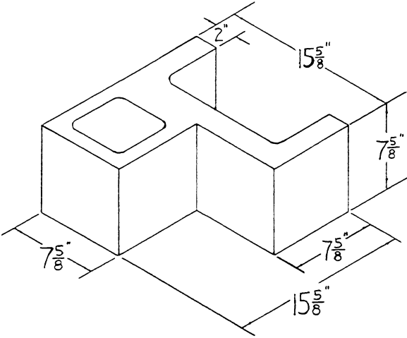
"H" PILASTER
