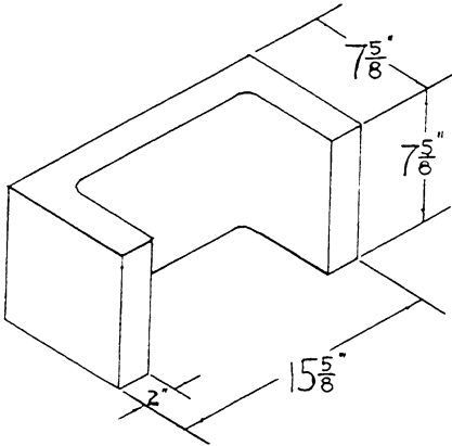
"C" PILASTER
