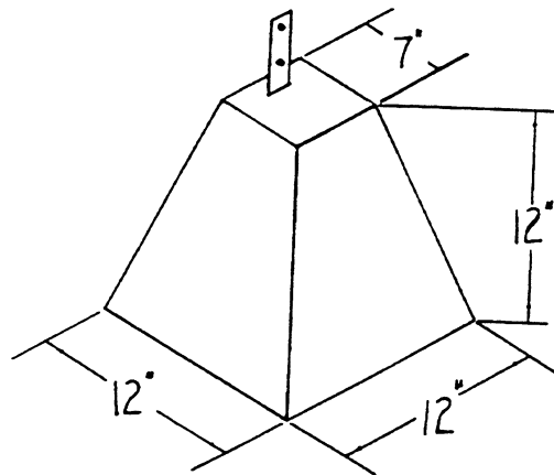
7 x 12 x 12 GARAGE PIER W/ STRAP
