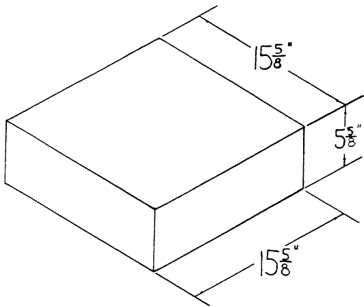
16×6×16 FOUNDATION BLOCK
