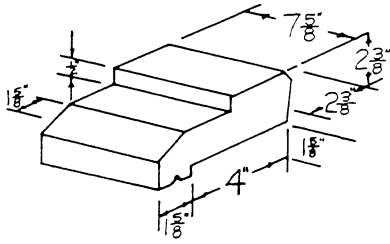
4" WINDOW SILL
