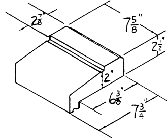
6" WINDOW SILL
