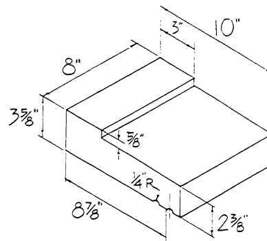
9" WINDOW SILL
