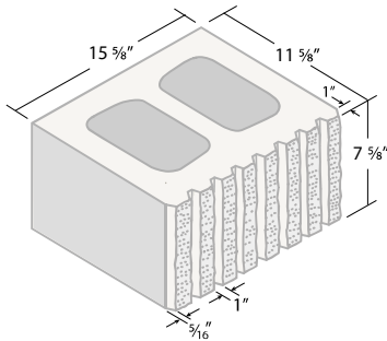
12 x 8 x 16 7V Fluted Split 1 Face** ITEM #0887V
