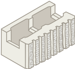
8x8x16 7-V FLUTED SPLIT BOND BEAM, 1 FACE
