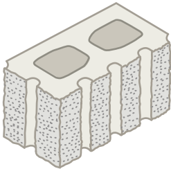
8x8x16 3-U FLUTED SPLIT 1 FACE/1 END
